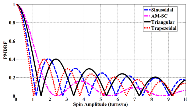
Fig. 4. PMDRF as a function of spin amplitude for four spin profiles, p = 1 m
