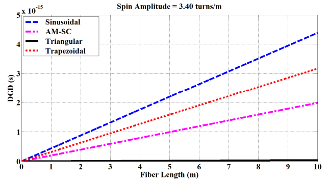
Fig. 6. DGD variation as a function of fiber length \alpha_0=3.40 turns/m, p=1 m, L_B=5 m
