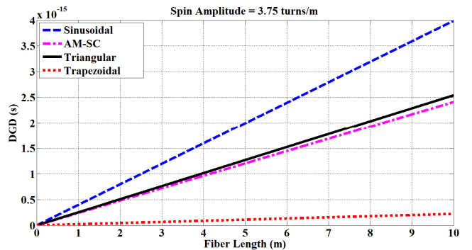
Fig. 7. DGD variation as a function of fiber length \alpha_0=3.75 turns/m, p=1 m, L_B=5 m
