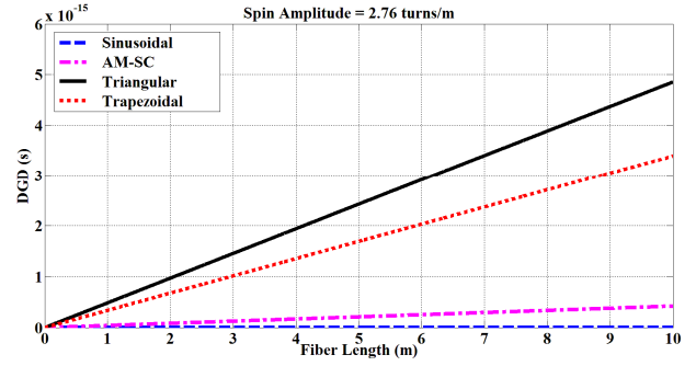
Fig. 5. DGD variation as a function of fiber length \alpha_0=2.76 turns/m, p=1 m, L_B=5 m
