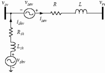
Fig. 2. Single phase representation of the UPFC system
