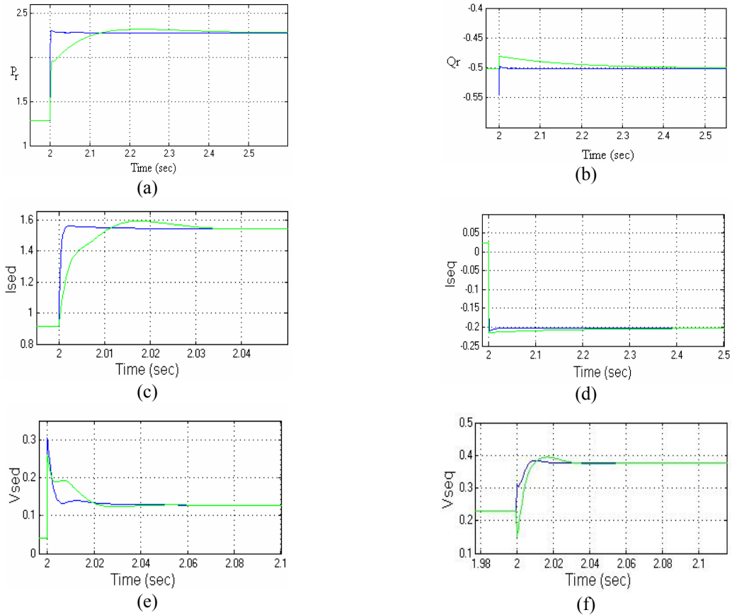
Fig. 5. Response of the UPFC system with 10% uncertainty according to the first case study
