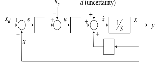
Fig 3. Schematic of system state space
