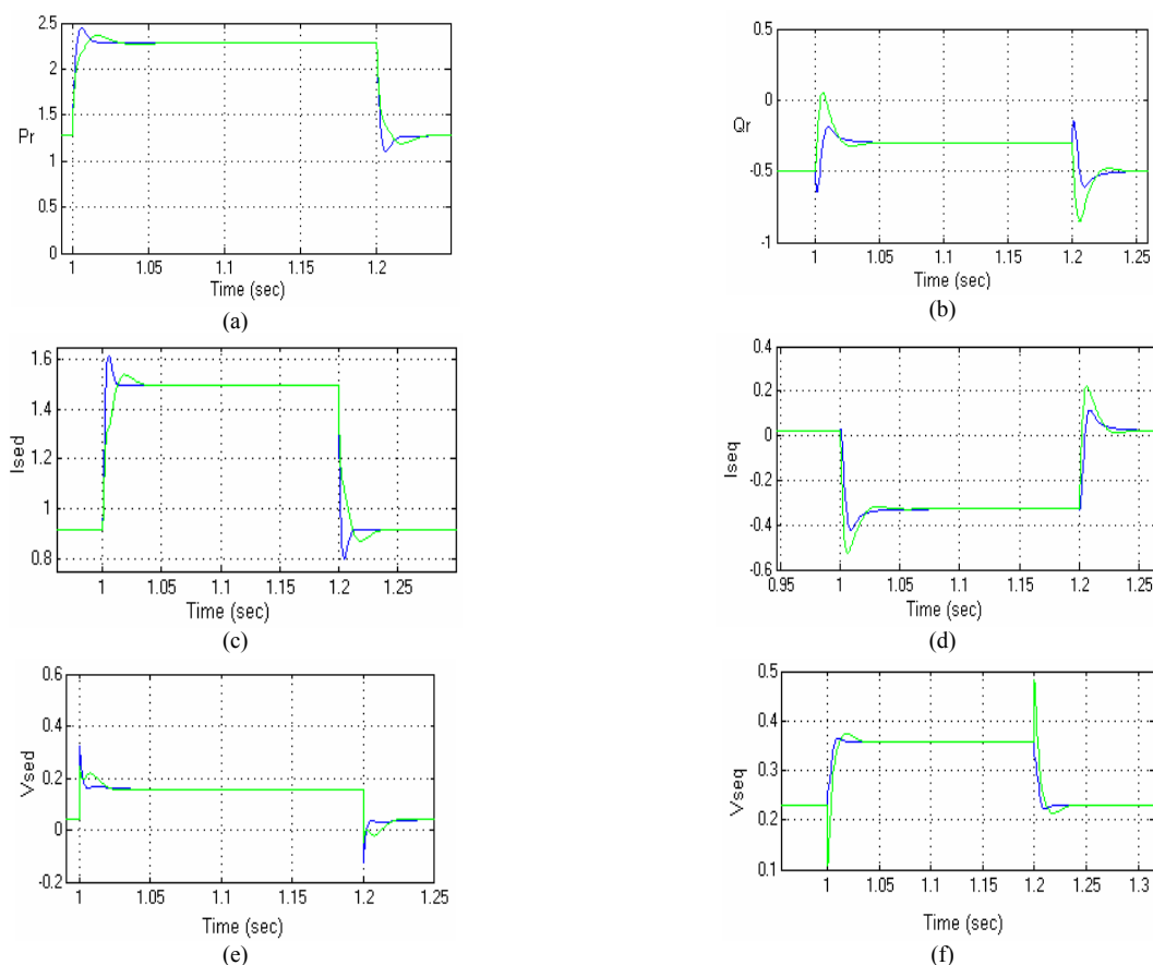
Fig. 7. Response of the UPFC system with 10% uncertainty according to the third case study
