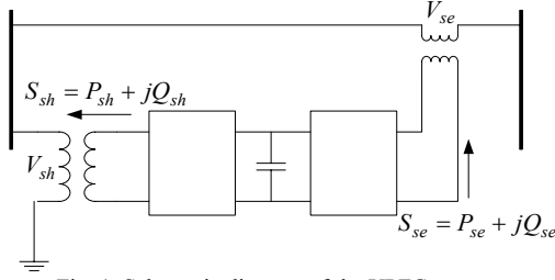
Fig. 1. Schematic diagram of the UPFC system
