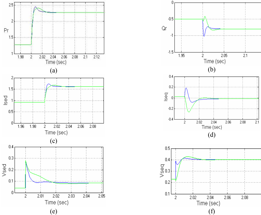
Fig. 6. Response of the UPFC system with 15% uncertainty according to the second case study
