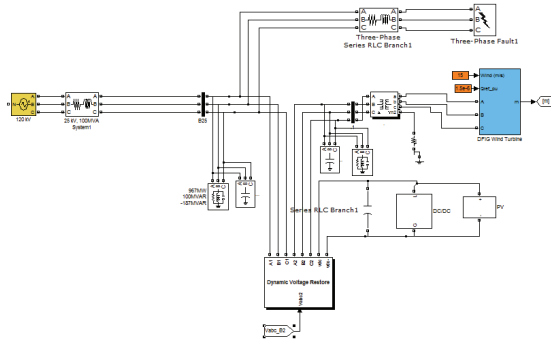
Fig.4. overall control circuit of DVR
