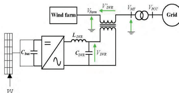
Fig.1. general system
