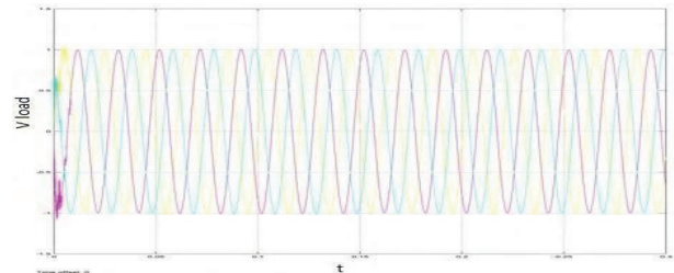
Fig.7. wind farm voltage in swell condition after compensation
