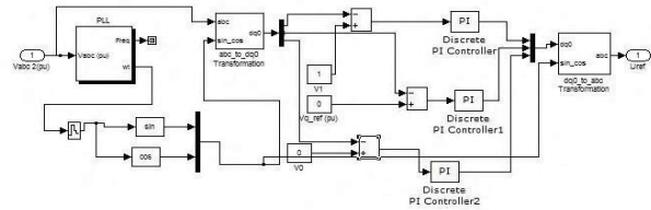
Fig.3. control block diagram for DVR
