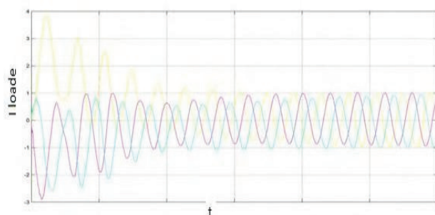
Fig.11. wind farm current after compensation (in both sag and swell condition)
