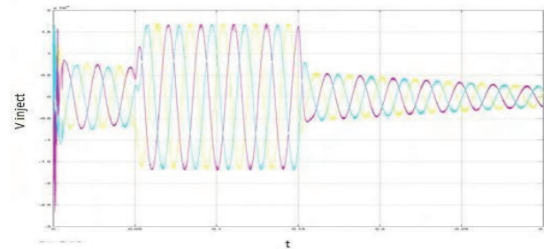
Fig.6. DVR injection voltage in swell condition
