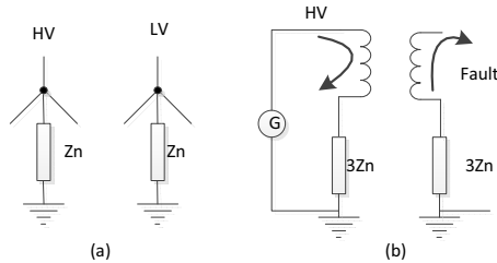
Fig. 3. YNyn Transformer zero sequence configuration
