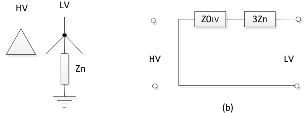
Fig.5. Δyn Transformer zero sequence configuration
