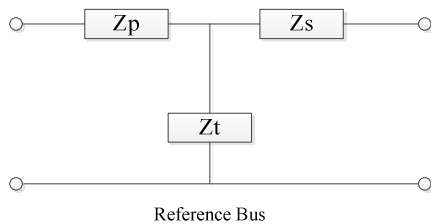
Fig.2. Transformer zero sequence Tee model diagram
