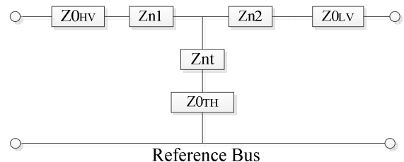
Fig. 7. YNa0d transformer zero sequence model
