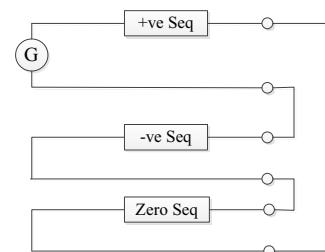
Fig.1. Sequence components connected in series
