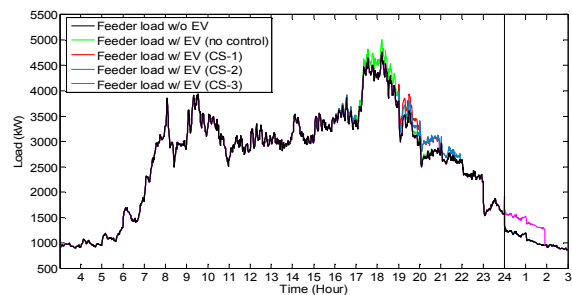
Fig. 7. Distribution system load profile without EV and with EV - quick charge - at 10% EV penetration level.
