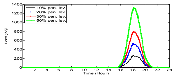
Fig. 3. EV load profiles – quick charge
