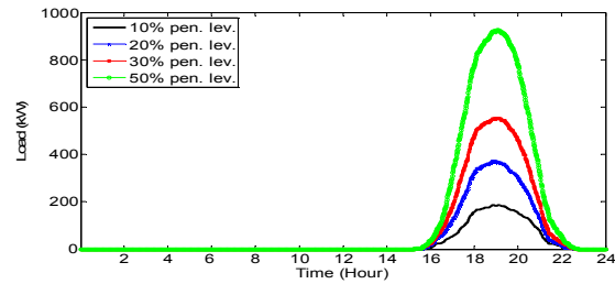
Fig. 2. EV load profiles – normal charge
