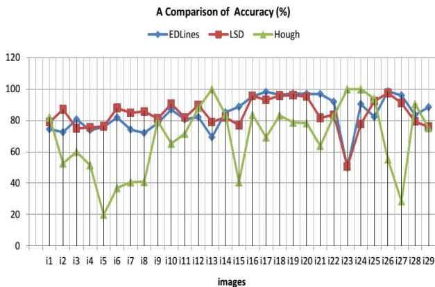
Fig 5. A Comparison of Accuracy (%)
