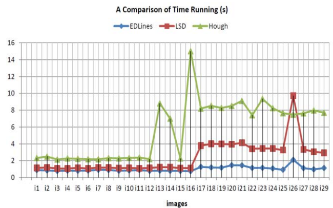
Fig 6. A Comparison of Run Time (second)
