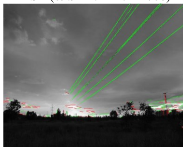
LSD (76.22-1.14-1024x768)
