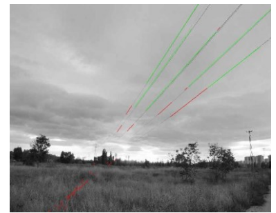
Hough (82.05-2.31-1024x768)
