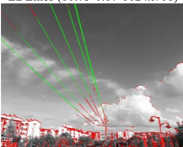
EDLines (88.76-0.78-1024x768)
