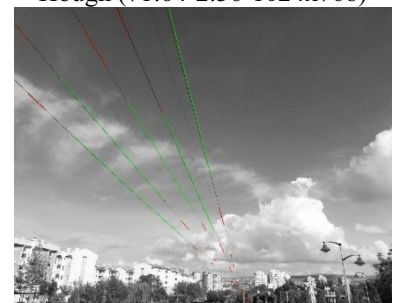
Hough (40.74-2.25-1024x768)
