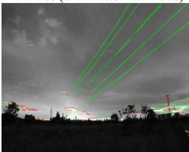
EDLines (75.89-0.77-1024x768)
