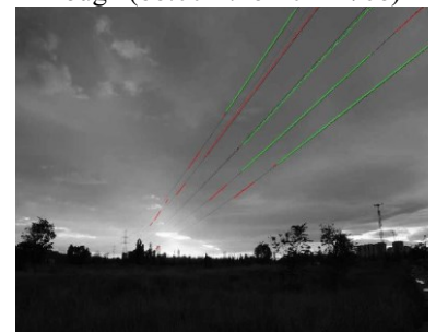
Hough (20.00-2.22-1024x768)
