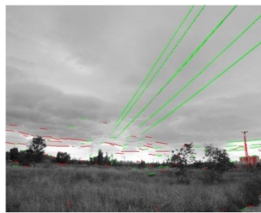
LSD (78.87-1.13-1024x768)
