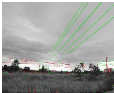
EDLines (74.51-0.88-1024x768)
