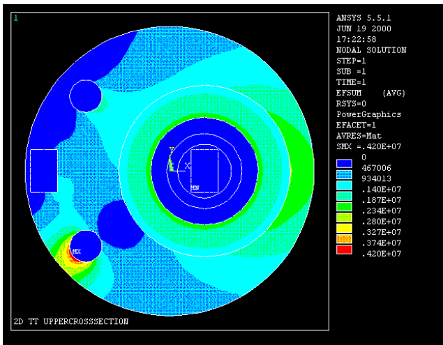
Figure 7. Upper view of electric field distribution of test transformer (for 95 kV).
