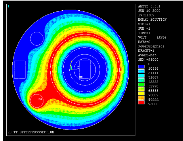
Figure 5. Dielectric field pattern in horizontal cross-section through centre of the HV bushing and HV outer layer when 95 kV is applied.
