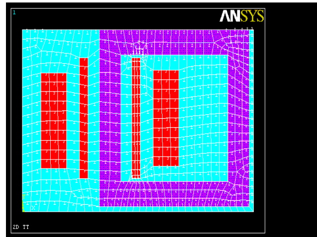
Figure 2. Finite element mesh of model.
