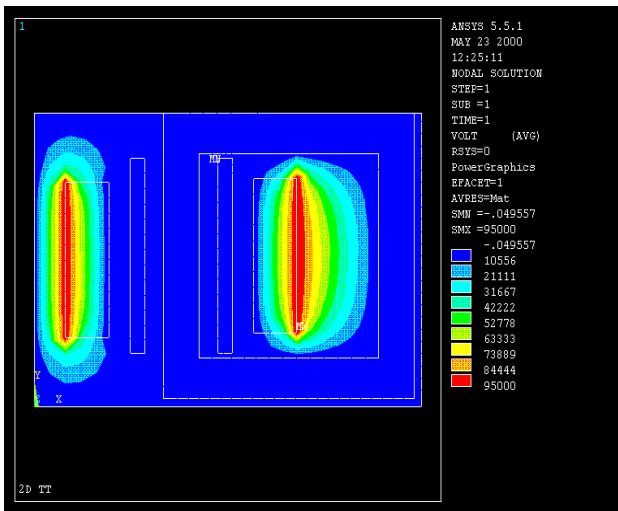
Figure 4. Test transformer equipotential lines for 95 kV.
