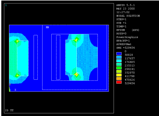
Figure 6. Electric field density when 95 kV is applied.
