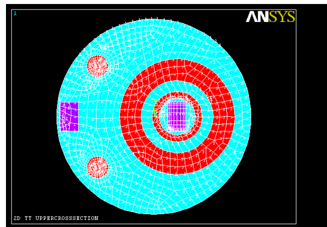
Figure 3. Element meshing in upper-view of test transformer.
