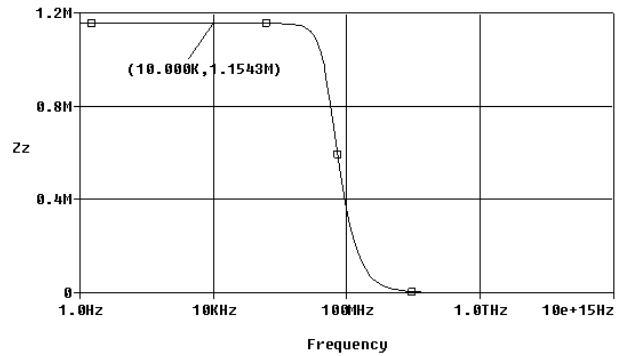
Fig. 10. The Z terminal output impedance.
