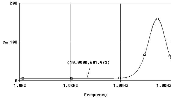
Fig. 12. The output Impedance of W terminal.
