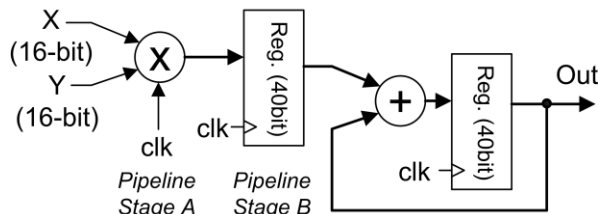
Fig. 5. Conventional MAC unit with various pipeline combinations
