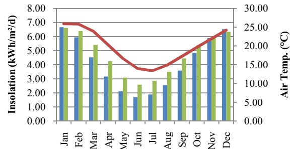
Fig. 4. Comparing horizontal and tilted panel insolation, and average maximum daily temperature
