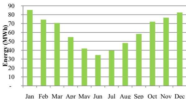
Fig. 5. Monthly energy generation for entire roof space.
