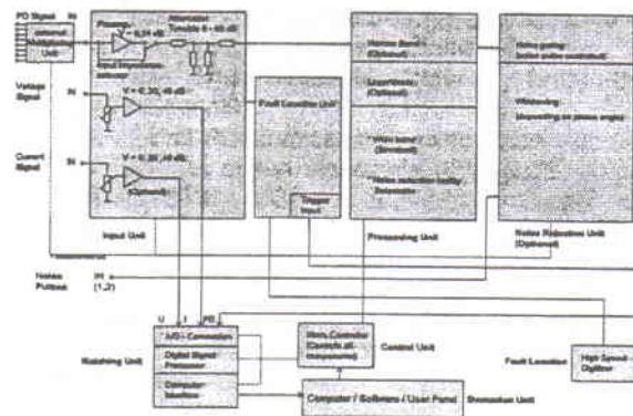
Figure 3: Schematic diagram of the PD-measuring unit
