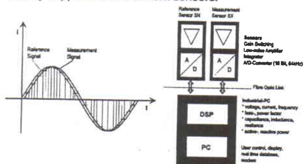
Figure 1: Concept of the loss / impedance measuring system
